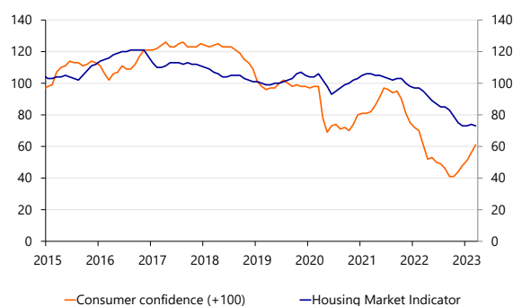
Chart 6: Confidence
