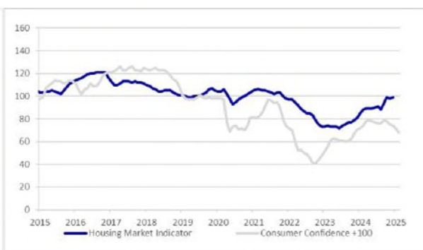
Chart 6: Confidence
