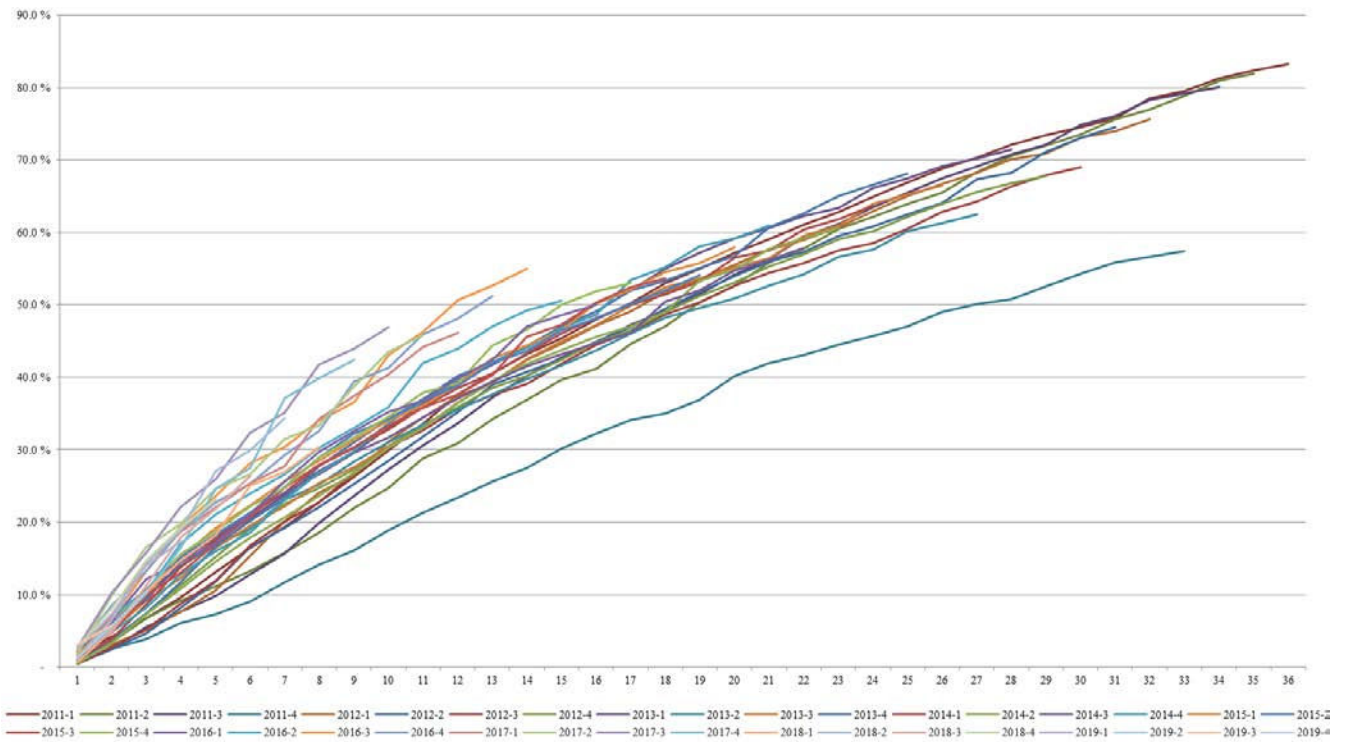
Cumulative recovery rate by vintage of default - eligible portfolio
