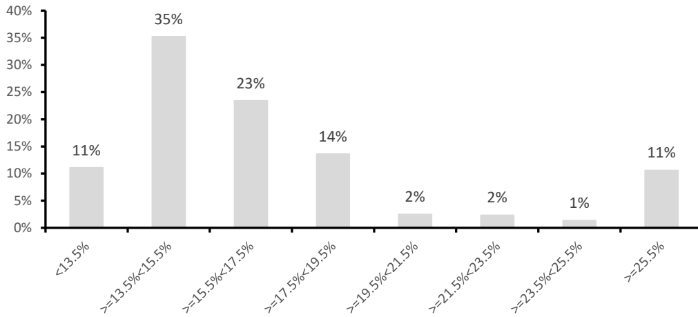
Distribution by average APR
